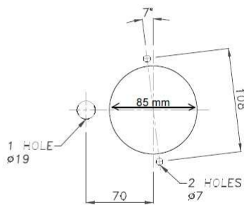
MOUNTING DETAIL
